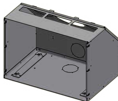
Cassette without cover plates in the top plate
